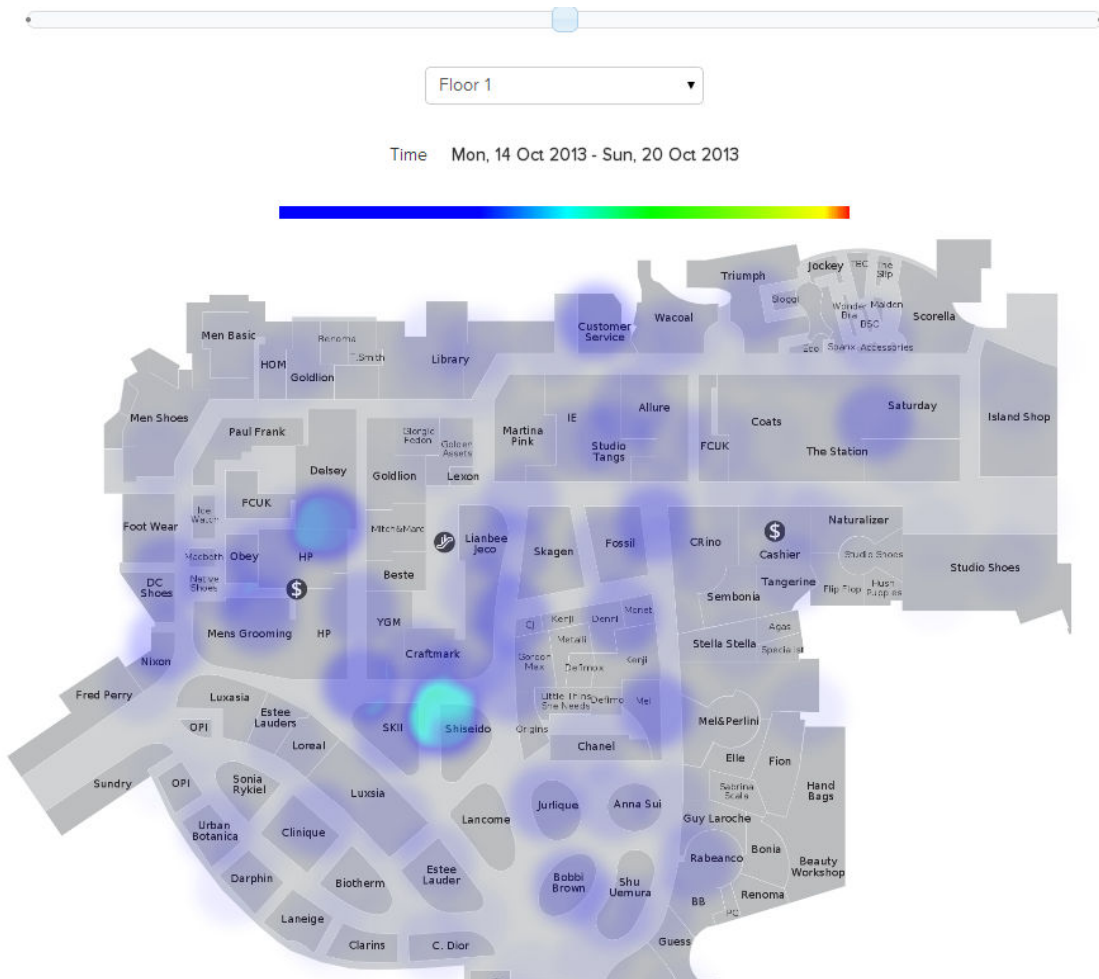
FIGURE 117 Heatmap
