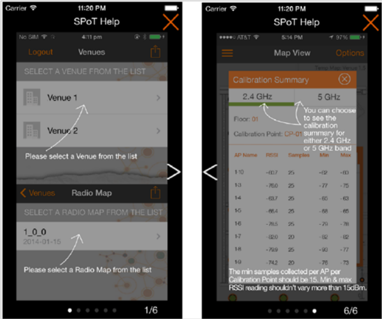
FIGURE 81 Help Screen
