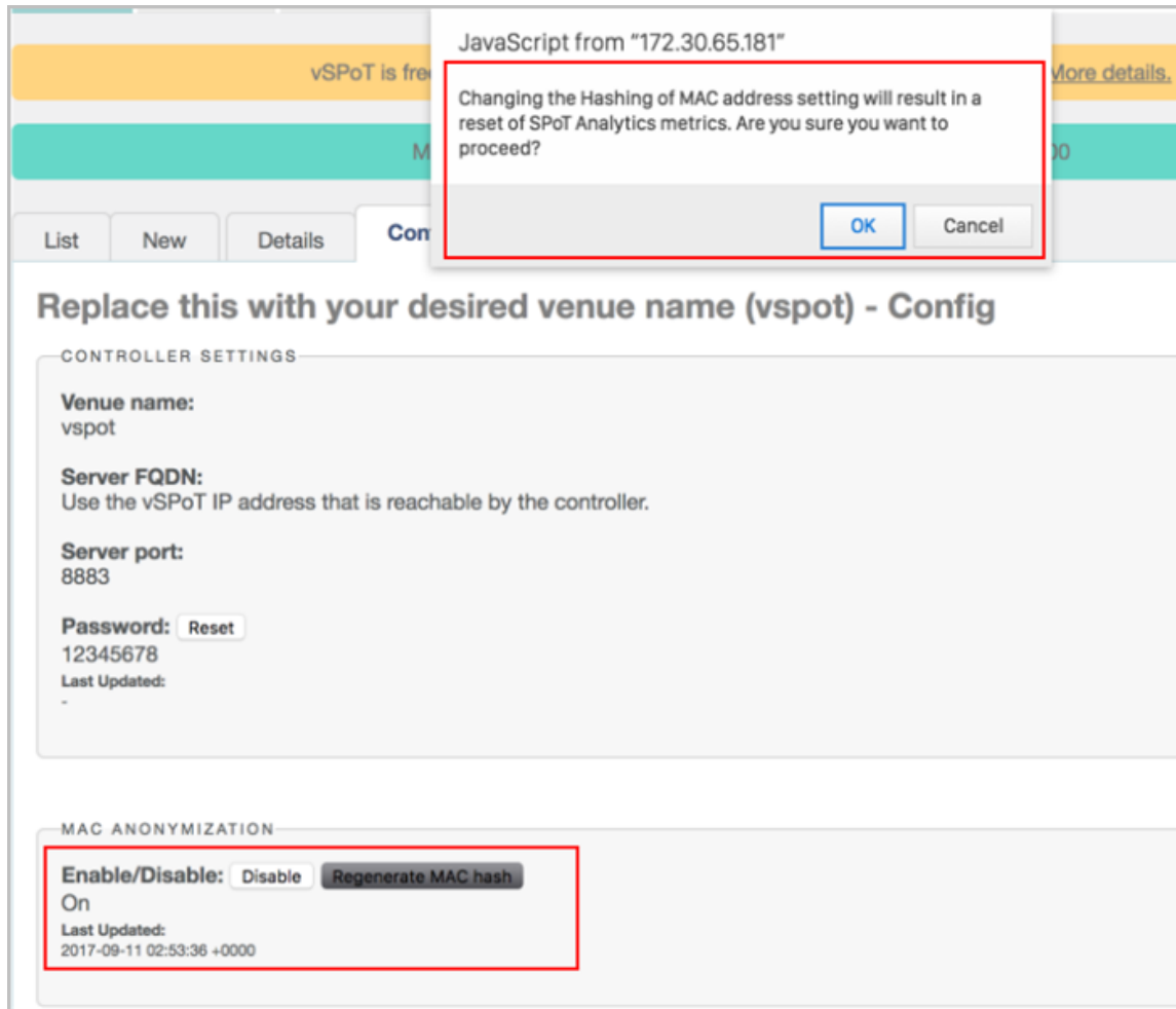
FIGURE 167 Using the regenerate MAC hash option
