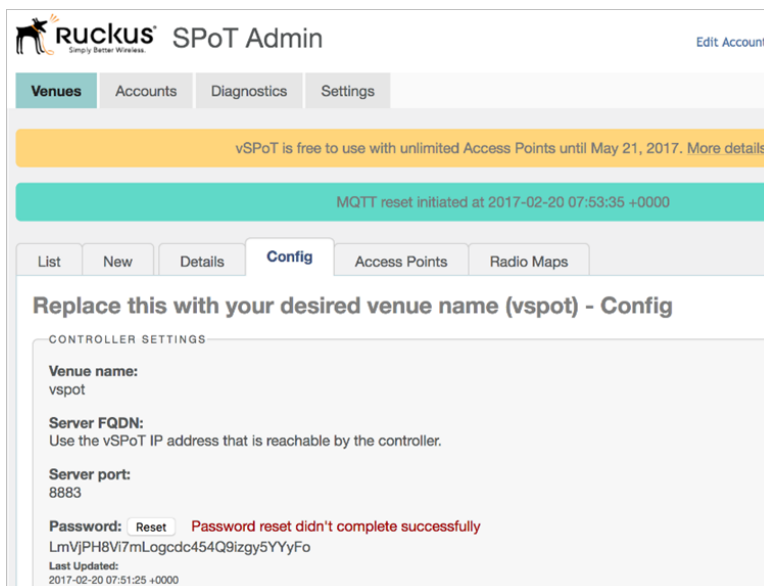
FIGURE 105 Failed MQTT PSK Update
