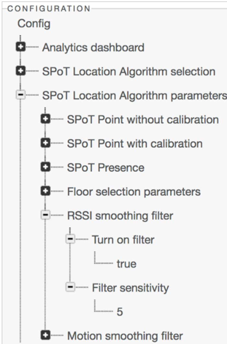
FIGURE 150 RSSI smoothing filter
