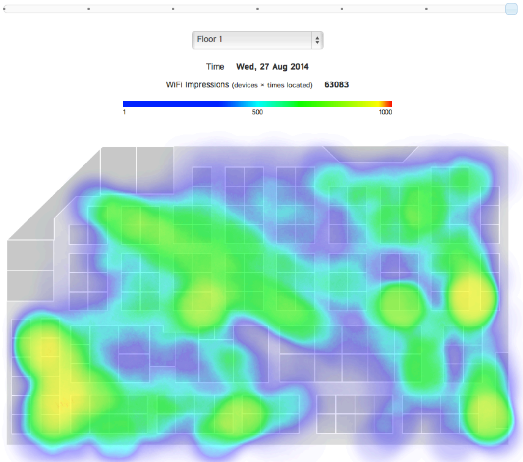
FIGURE 138 Heatmap bubble radius of 3000mm and colorbar maximum of 1000.
