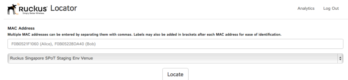
FIGURE 125 Enter MAC addresses of clients to track
