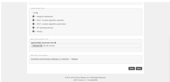
FIGURE 129 Use the Device Catalogue section on the Admin Portal Config page to manage the device MAC address list for real-time tracking
