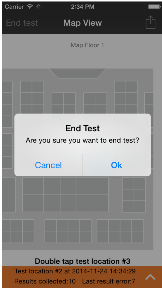
FIGURE 87 End Test
