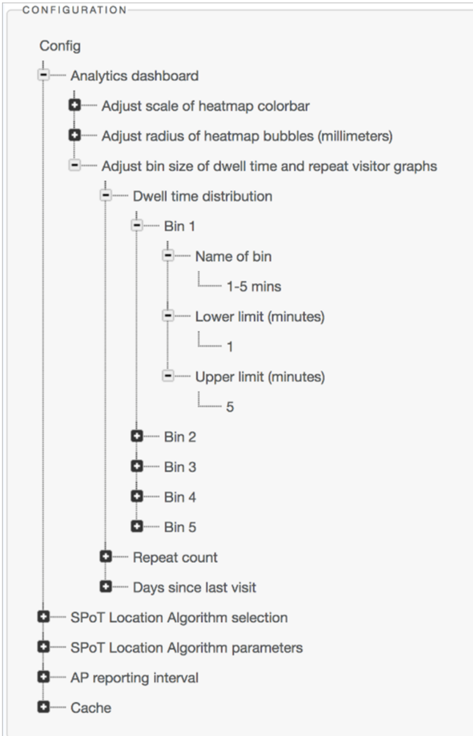
FIGURE 141 Configuring the bin sizes
