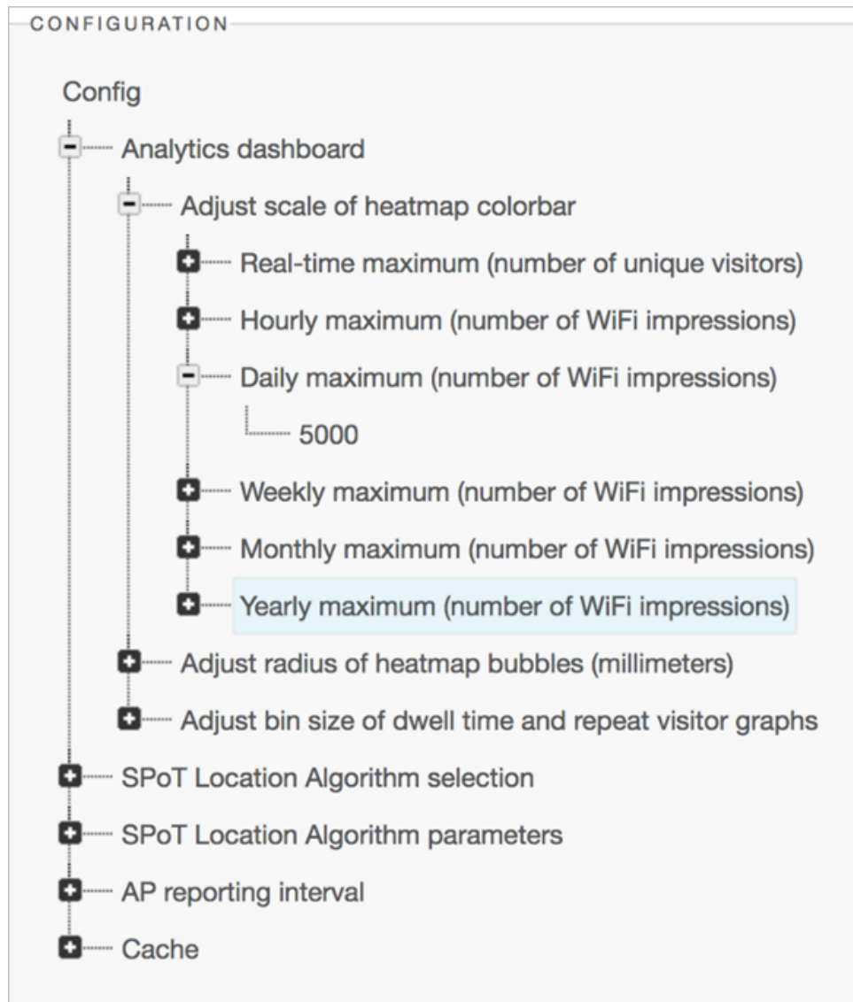
FIGURE 134 Adjusting colorbar maximum for various heatmaps
