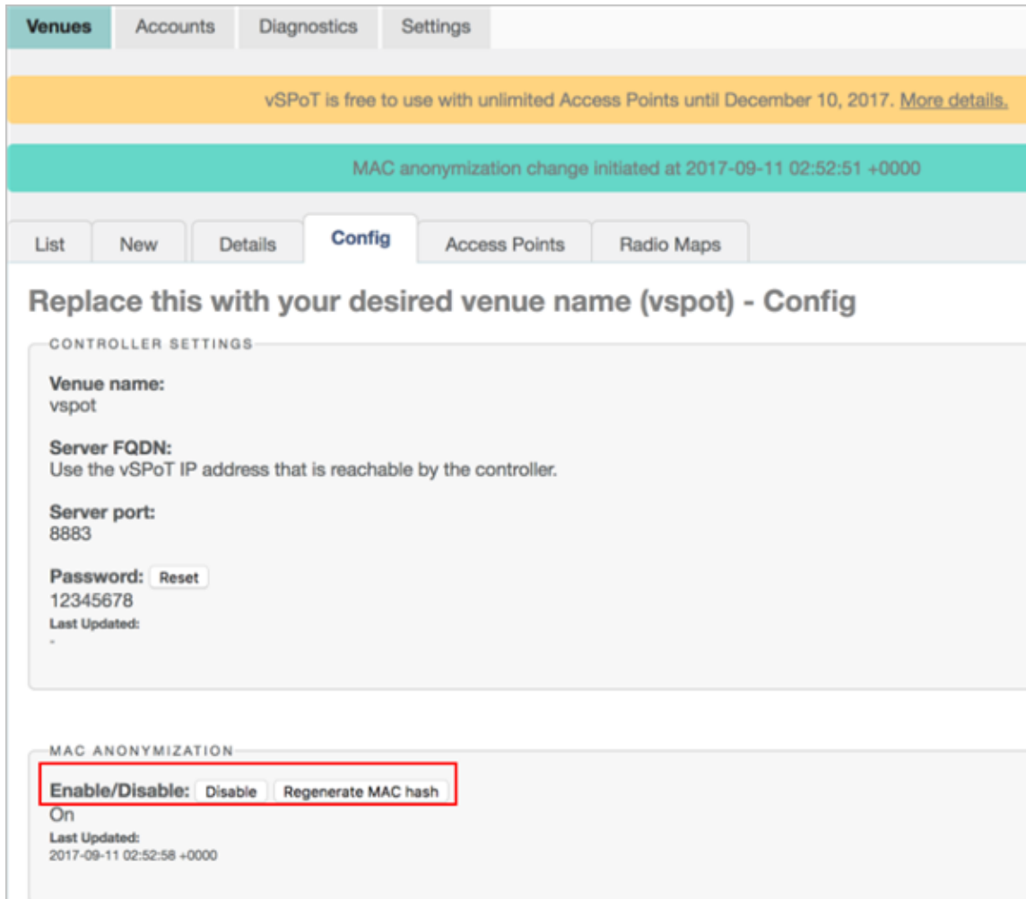
FIGURE 166 Selecting MAC Anonymization
