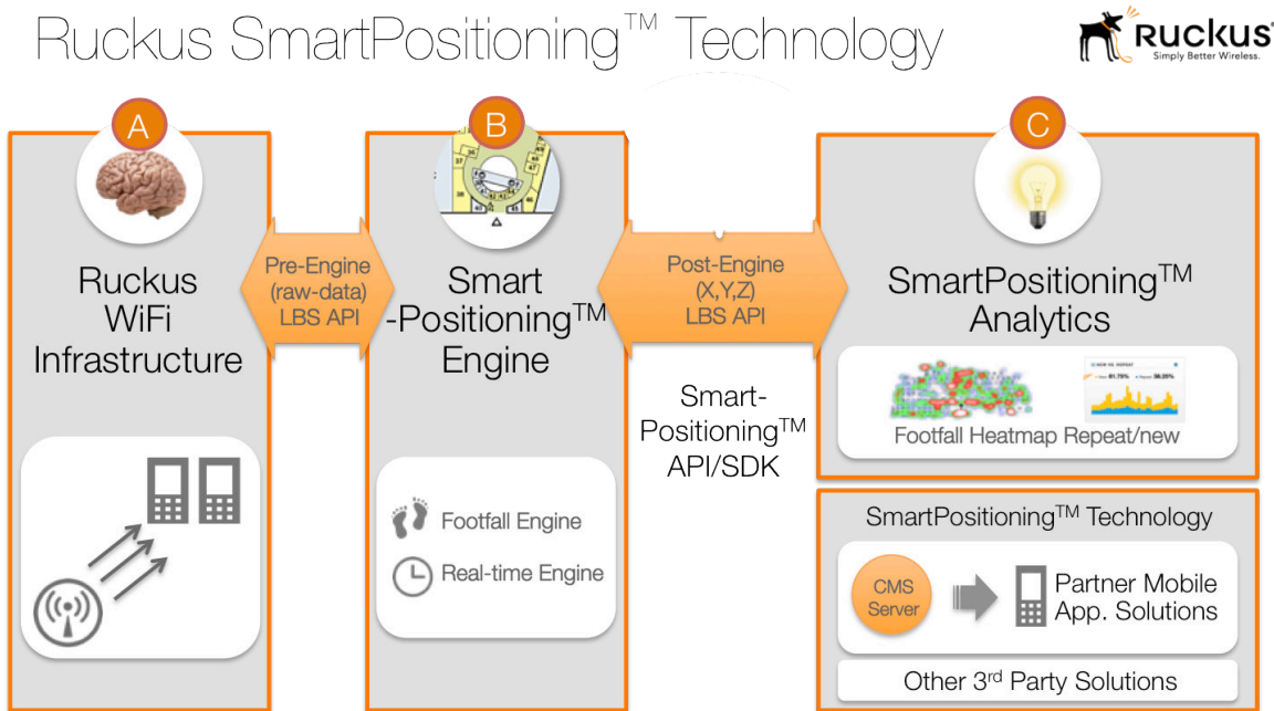
FIGURE 1 SmartPositioning high level architecture
